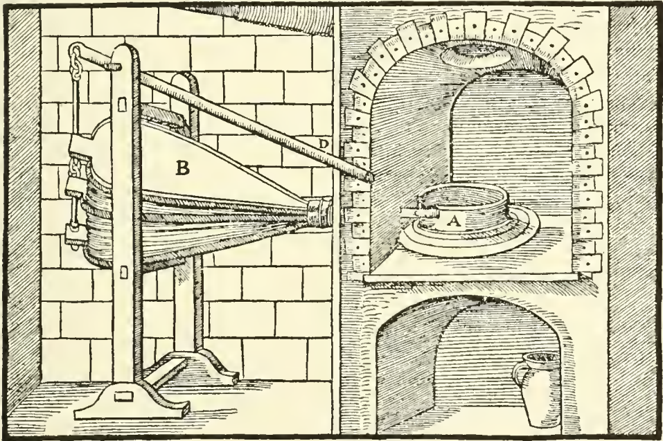
A—IRON HOOP. B—DOUBLE BELLOWS. C—ITS NOZZLE. D—LEVER.
